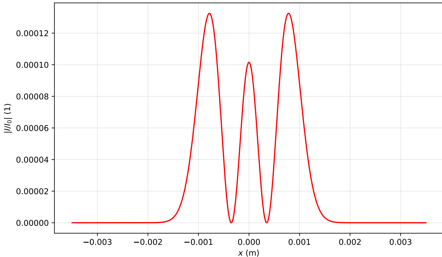
Intensity profile I(x, y = 0, z = 0.080)/I_0 , P_{in}=2.0P_{cr} , artificial time
